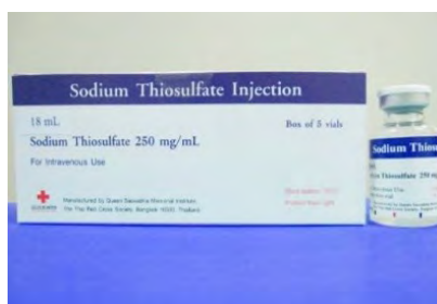
25% Sodium Thiosulfate
